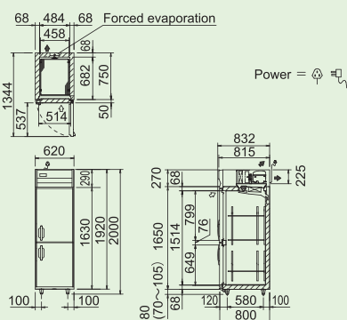
SRR-681HP(E)
